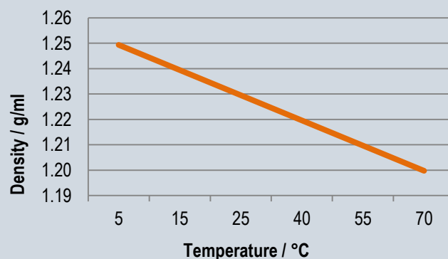
TERATE® HT 5510 Density – Temperature Data
