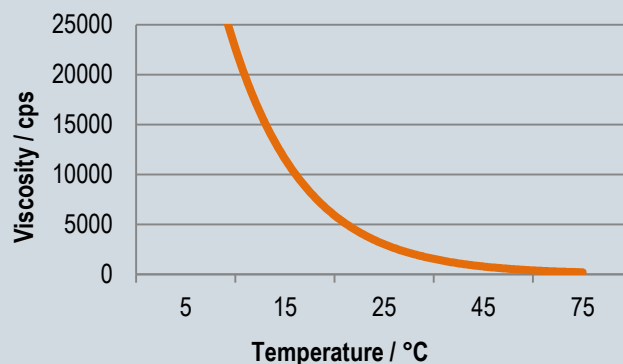
TERATE® HT 5510 Viscosity – Temperature Data
